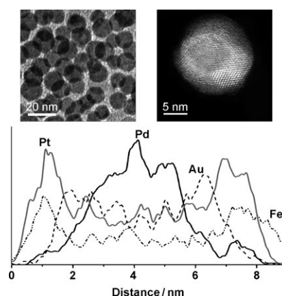
Figure 2. a,b) Representative TEM (a) and HR-STEM (b) image of a single 5/1/2 nm Pd/Au/FePt NP. c) High-resolution line-scan EDS analysis across the NP. The analysis was obtained by scanning 150 points with a beam size of about 2 Å.
