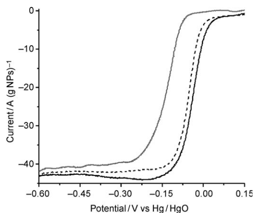
Figure 4. Polarization curves showing the oxygen reduction reaction current for three different Pd/Au NPs having 1 nm (—), 1.5 nm (---), and 2 nm (— · —) coatings. The current was standardized against the total mass of NPs (40 \mu\text{g} ) used, and the electrode rotation rate was kept at 1600 rpm.
